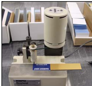
Using a piece of scrap makes "pushing" your small material through the beveler easier.
